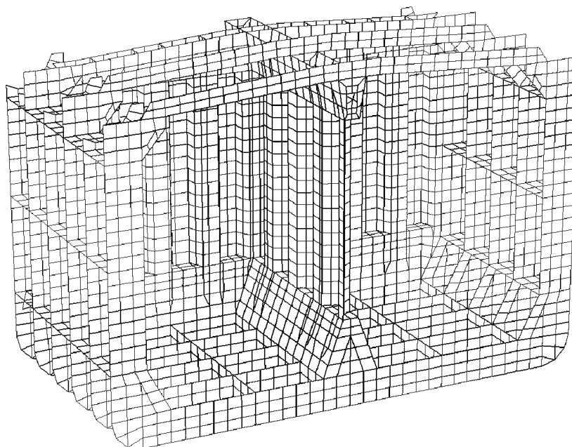
Product tanker
