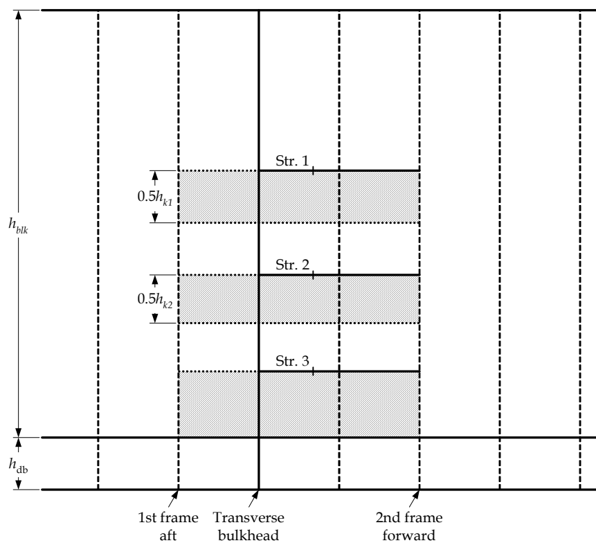
Figure 8.1.7 Load Breadth of Stringers for Ships with a Centreline Bulkhead
