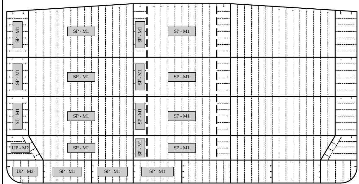
Figure D.5.3 Transverse Bulkhead
