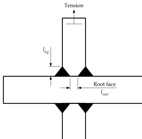
Figure 6.5.11 Welds Subject To High Tensile Stresses
