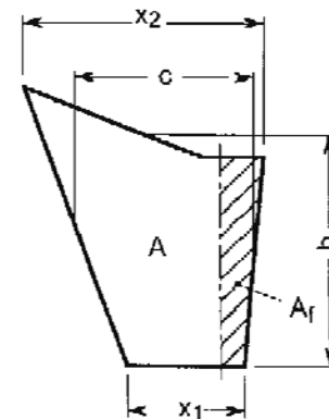
Figure 18.1 Rudder area geometry
