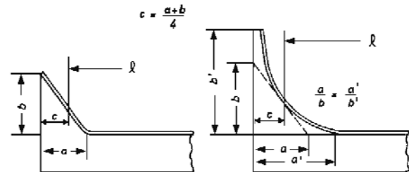
Figure 3.3 Unsupported span \ell
