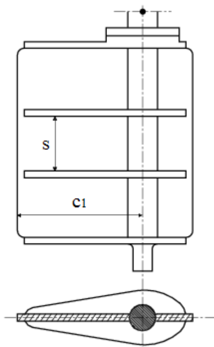
Figure 18.10 Single Plate Rudders
