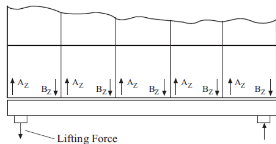
Fig. 15.9 Lifting forces at a hatch cover
