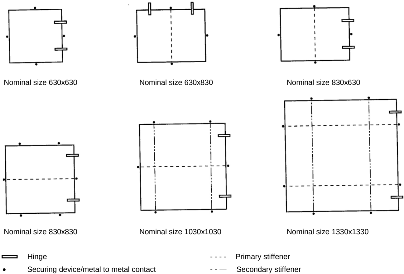
Figure 15.11 Arrangement of stiffener
