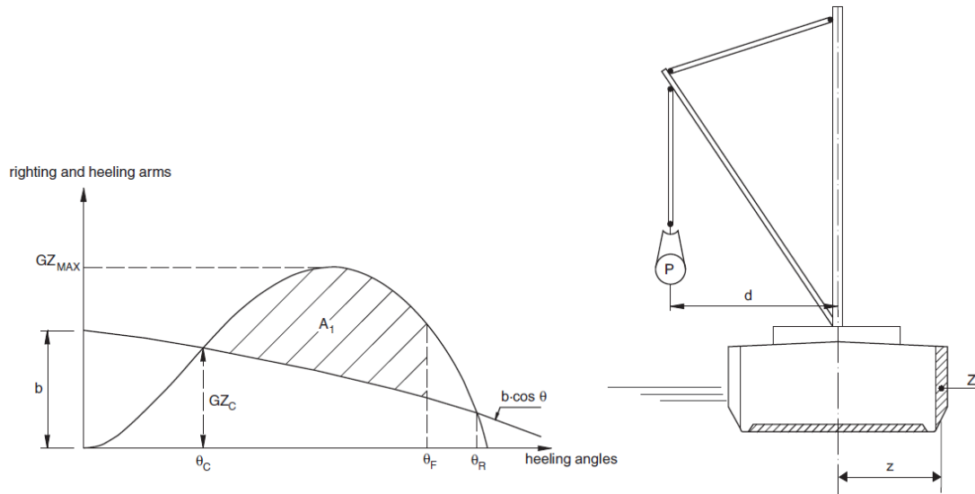
Figure 26.2 Cargo Lifting
