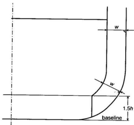
Figure 28.3 Cargo tank boundary lines for the purpose of item 2.2.1.1.2 - Guidance
