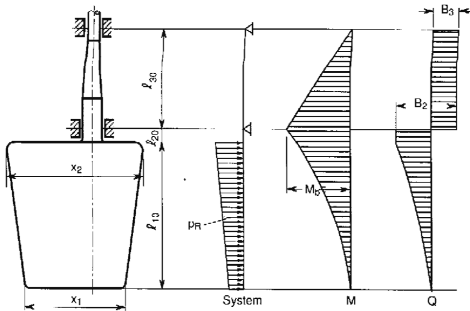
Figure 18.5 Spade rudder
