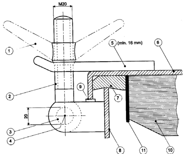
Figure 15.11 Arrangement of stiffener
