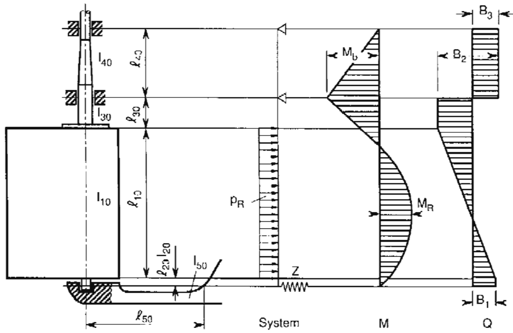
Figure 18.3 Rudder supported by sole piece
