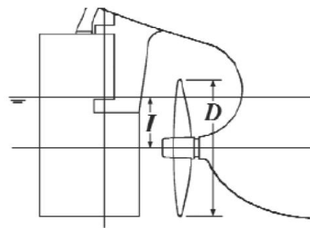
Figure 6.13 Propeller Immersion
