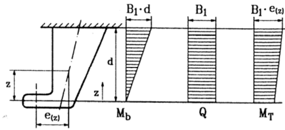
Figure 10.6 Loads on the rudder horn
