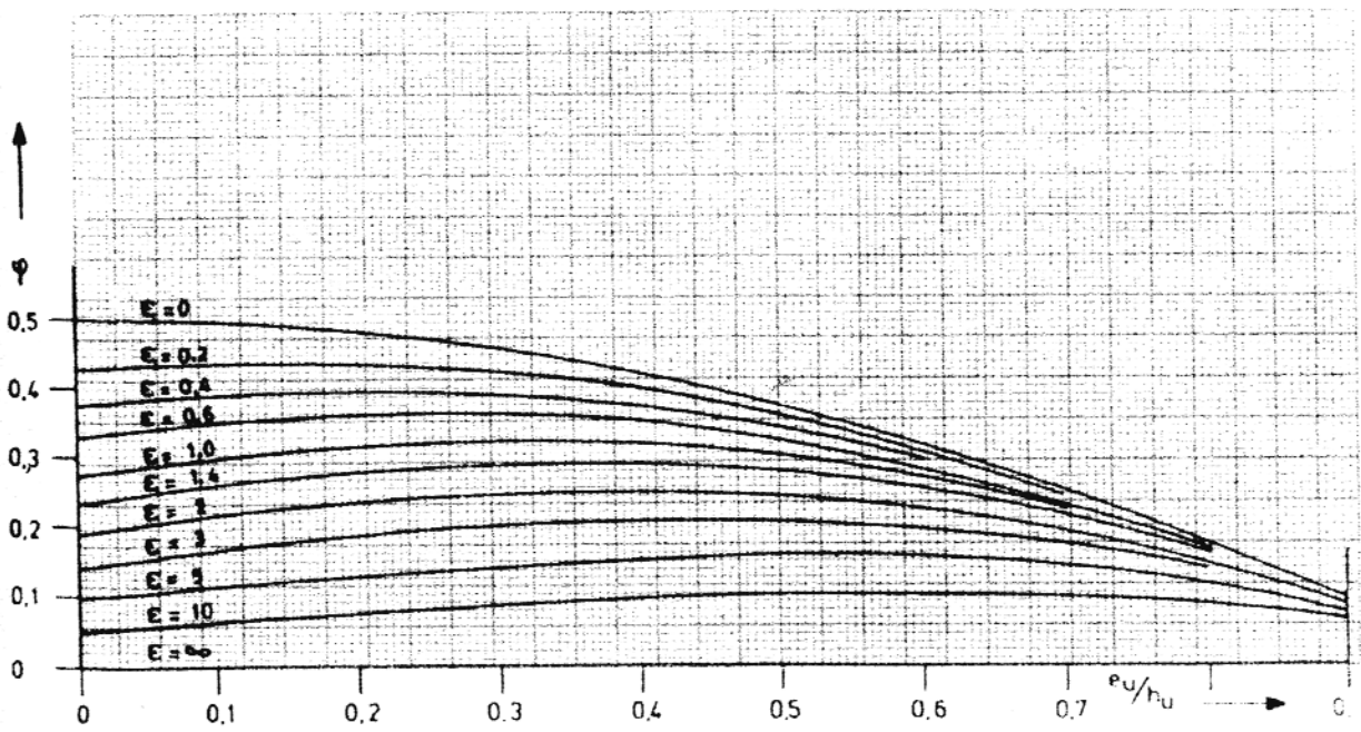
Diagram 8.2 coefficient \varphi
