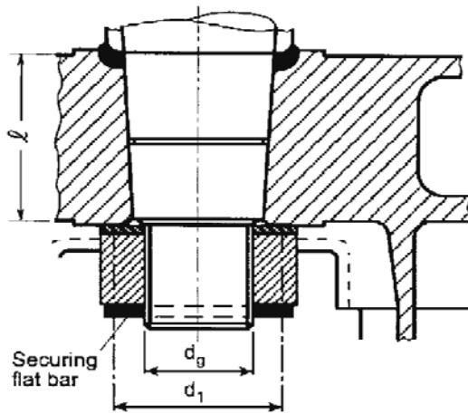
Figure 18.8 Cone coupling without key and with securing flat bar
