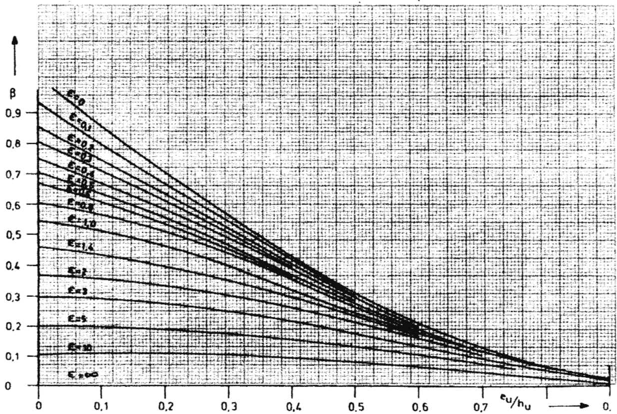
Diagram 8.3 coefficient \beta
