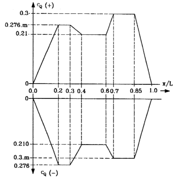
Figure 6.3 Distribution factor C_Q
