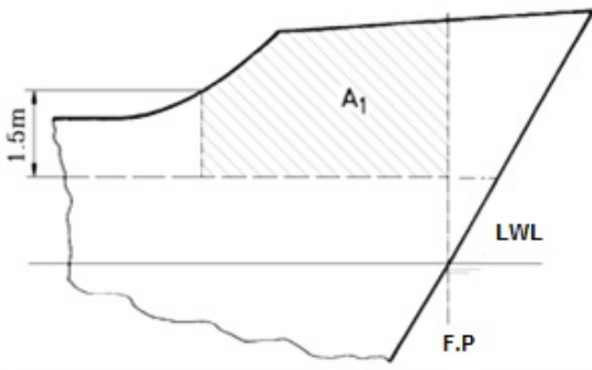
Figure 17.1 Effective area A_1 of bulwark
