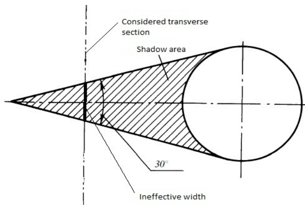
Figure 6.7 Shadow area
