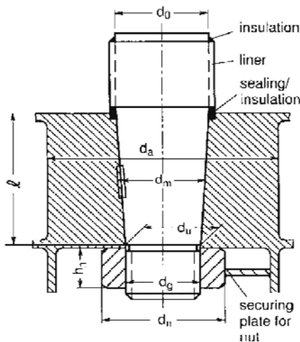
Figure 18.7 Cone coupling with key and securing plate
