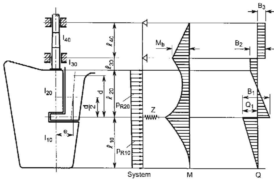
Figure 18.4 Semi-spade rudder
