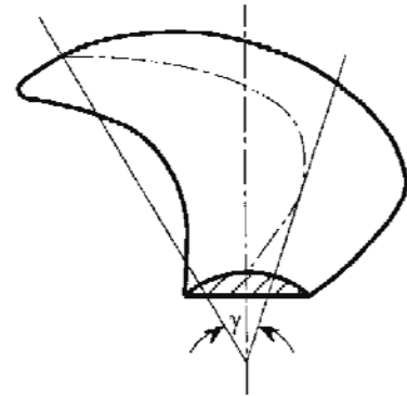
Figure 10.2 Skew angle
