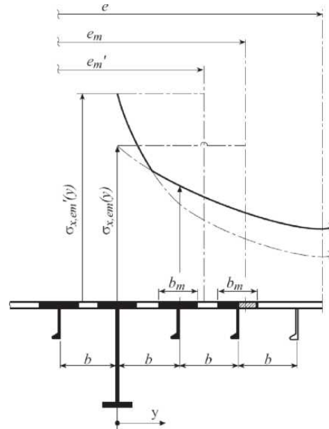
Fig. 15.6 Stiffening parallel to web of primary supporting member
