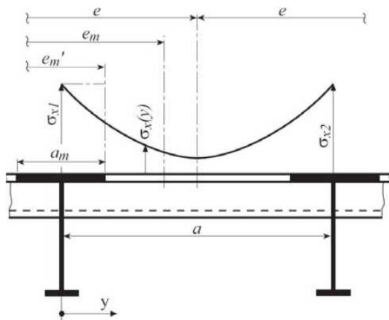
Fig. 15.7 Stiffening perpendicular to web of primary supporting member
