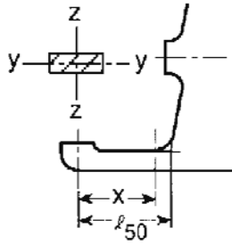
Figure 10.4 Length l_{50} of a sole piece
