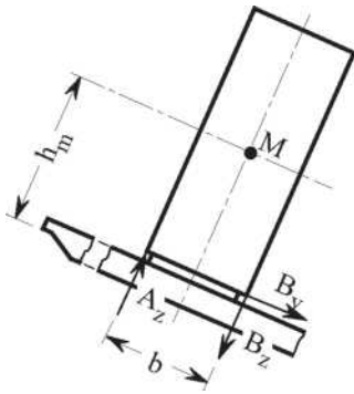
Fig. 15.3 Forces due to load case C acting on hatch cover
