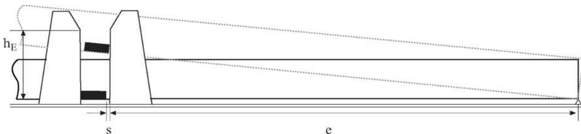
Fig. 15.10 Height of transverse cover guides
