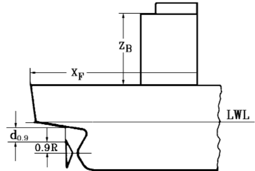
Figure 10.1 Propeller clearance d_{0,9}
