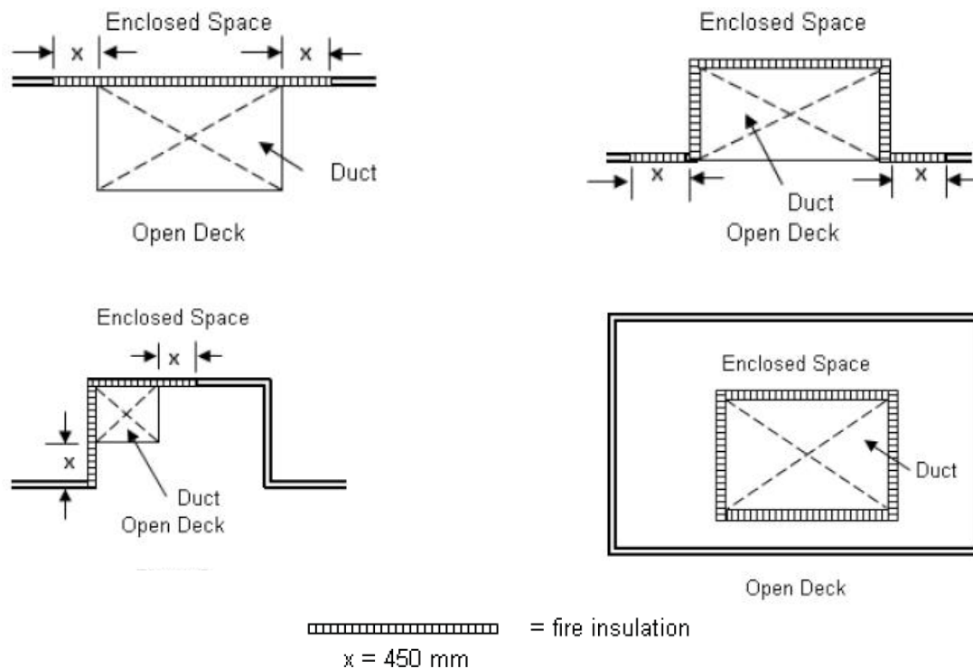
Figure 21.1 Examples of galley ducts contiguous to enclosed space
