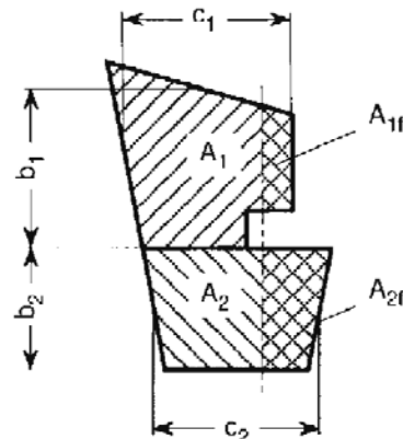
Figure 18.2 Partial rudder areas A_1 and A_2
