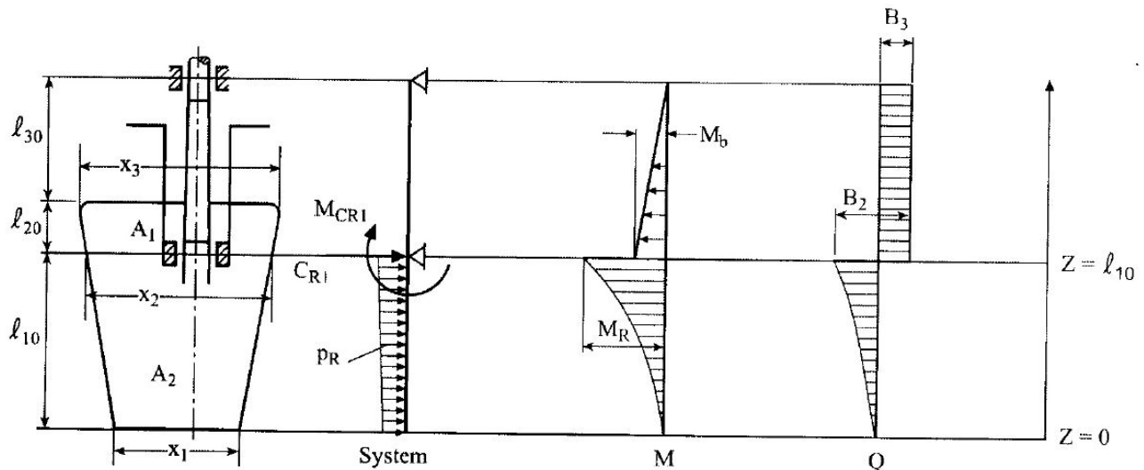
Figure 18.5 Spade rudder
