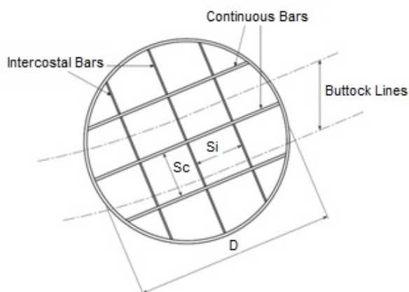
Figure 15.5 Standard construction of lateral thruster grid
