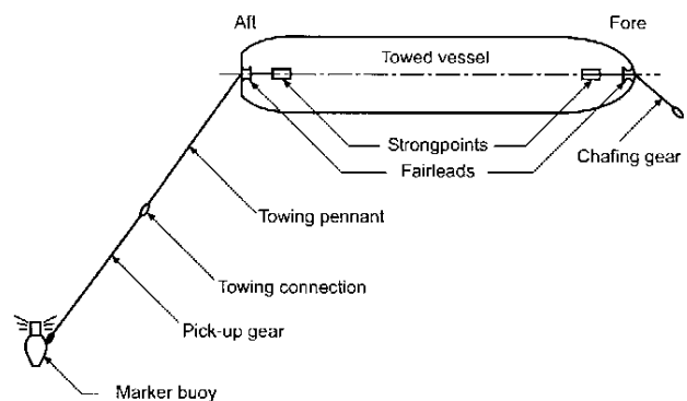
Figure 28.4 Typical emergency towing arrangement
