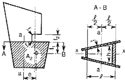
Figure 18.9 Geometry of a semi-spade rudder
