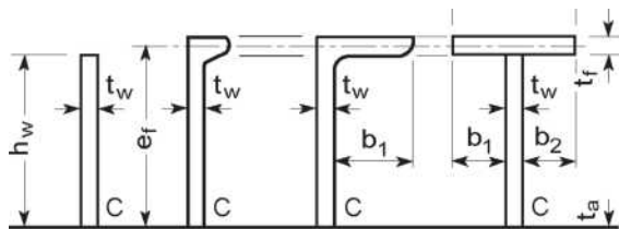
Fig 15.8 Dimensions of stiffener
