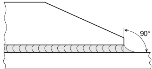
Fig. 16.3 Welding round of stiffening plates or web plates
