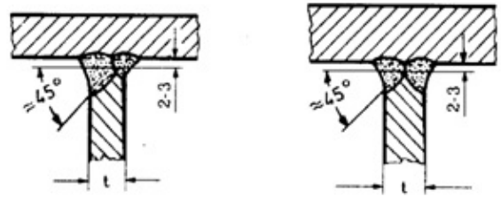
Fig. 12.22 Single- and double-bevel welds with full root penetration
