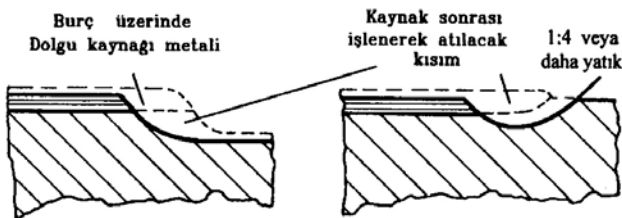
Fig. 12.18 Build-up welds applied to rudder-stocks and pintles
