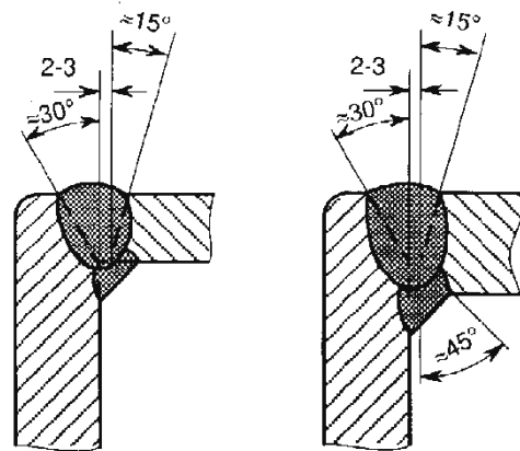
Fig. 12.26 Flush fitted corner joints
