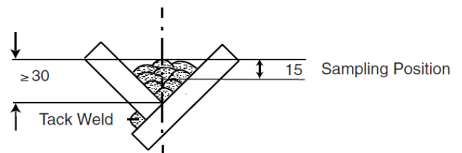
Figure 5.13 Deposited weld metal test assembly
