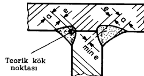
Fig. 12.28 Fillet welds with increased penetration
