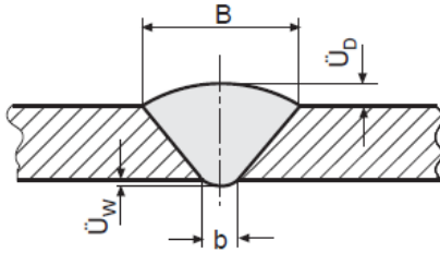
Fig. 15.1 Weld reinforcements
