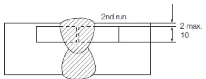
Figure 5.10 Test specimens
