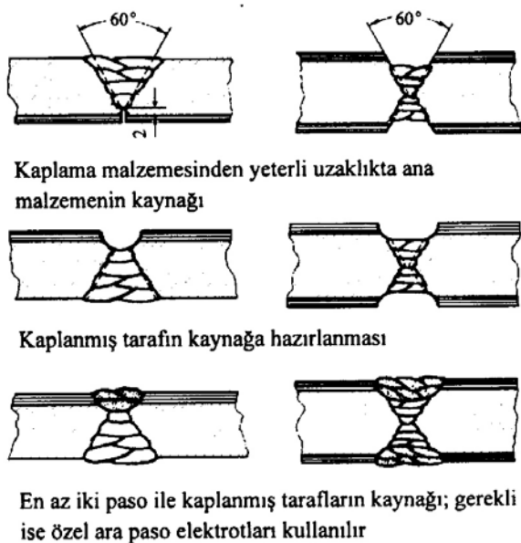
Fig. 12.21 Weld shapes for welding of clad plates
