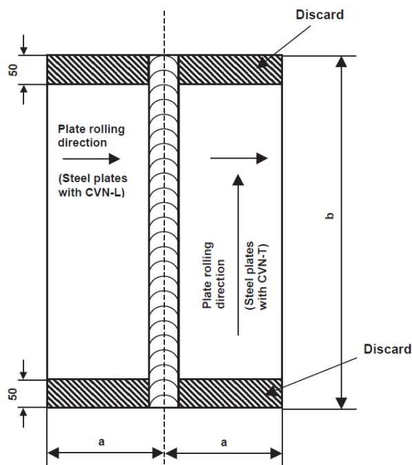
Figure 12.1 Test assembly for butt weld
