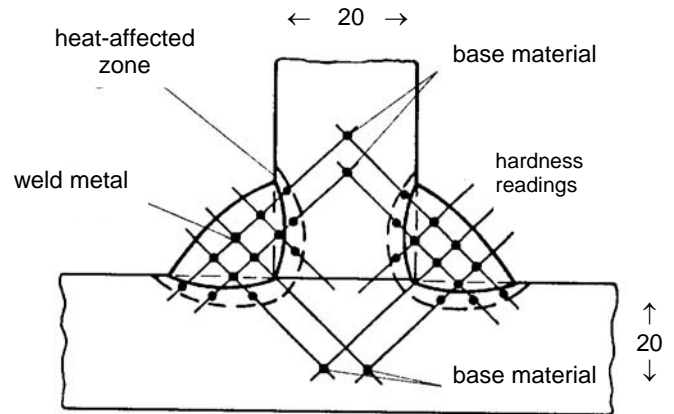
Figure 5.5 Hardness measurements
