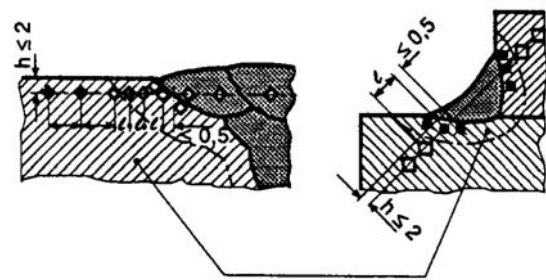
Heat-affected zone
