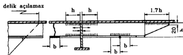
Fig. 12.30 Welds at the ends of girders and stiffeners
