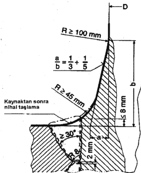
Fig. 12.36 Welded joint between rudder shaft and coupling flange
