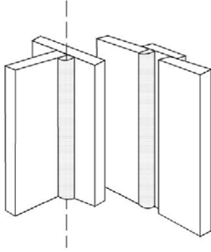
(C) VERTICAL POSITION 3F
