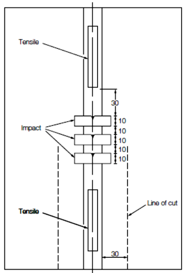
Figure 5.7 Preparation of one deposited metal test assembly
