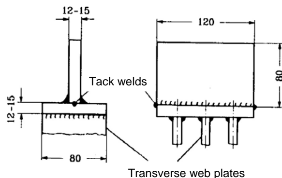
Figure 5.4 Test piece for hot cracking
