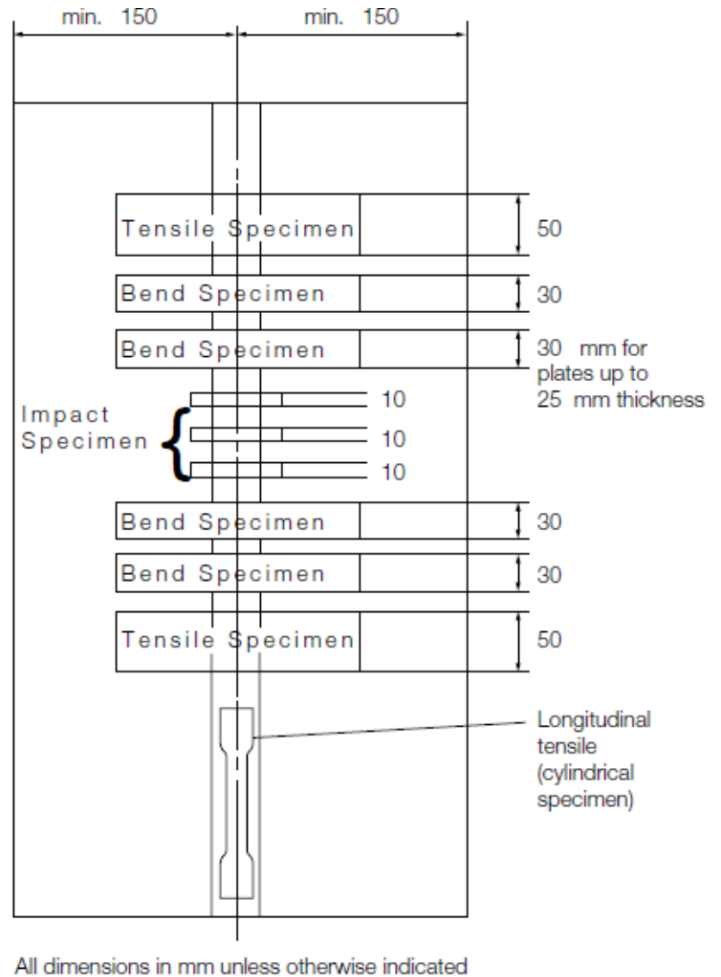
Figure 5.10 Test specimens
