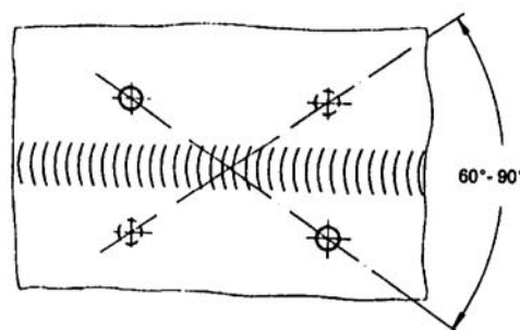
Figure 10.4 Directions in which magnetization is to be effected
