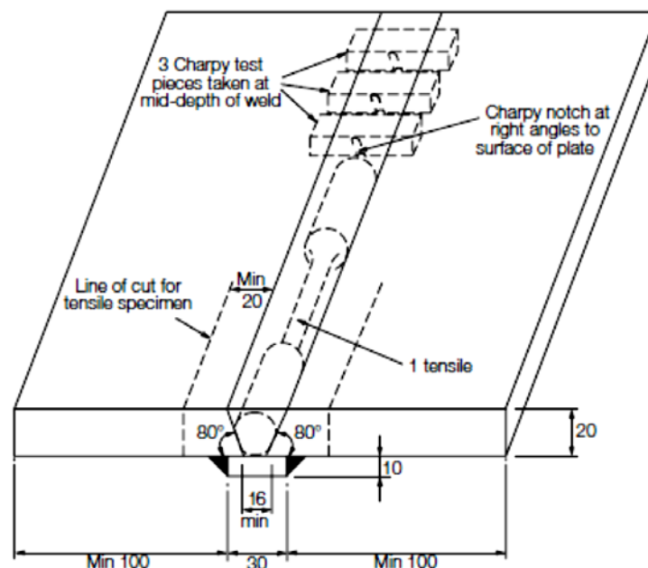
Figure 5.1 Weld metal test piece
