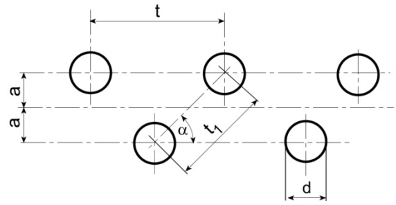
Figure 12.23 Length of ligament for staggered rows of holes
