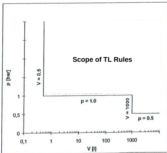
Fig. 14.1 Scope of TL Rules for pressure vessels and heat exchangers
