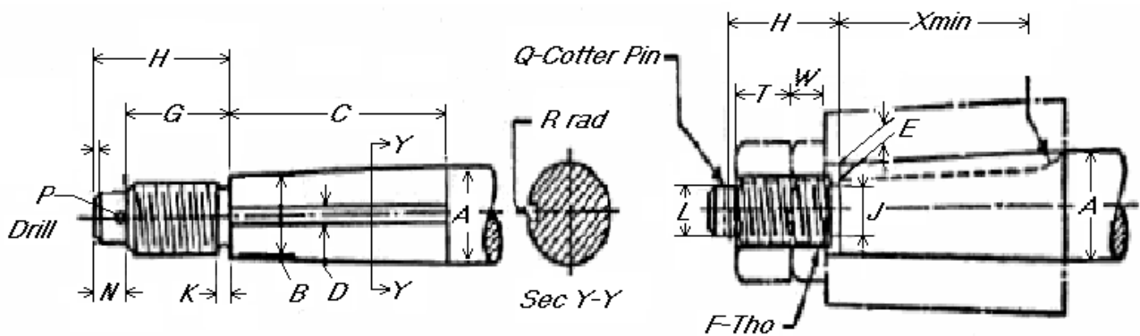
Figure 5.2 Typical details of propeller shaft ends
