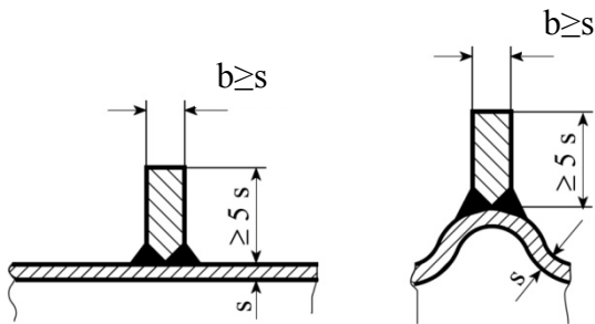
Figure 12.4 Effective stiffening
