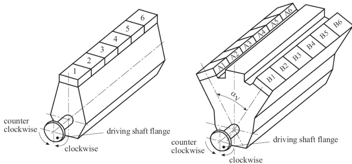
Fig. 2.1 Designation of the cylinders
