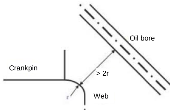
Fig. 2.7 Oil bore proximity to fillet
