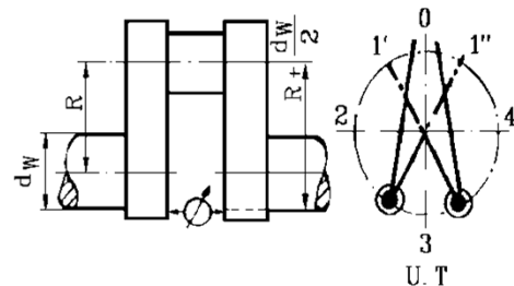
Fig. 2.19 Measurements of crank web deflections
