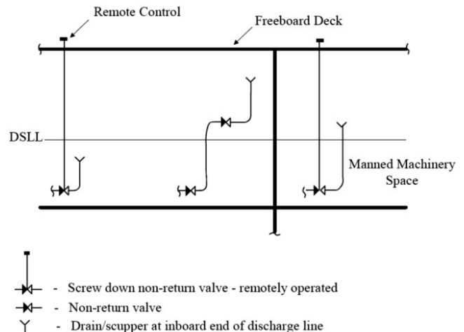
Figure 16.4 Overboard discharges from spaces below freeboard deck and valve arrangements according to SOLAS
