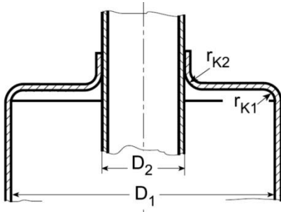
Figure 12.21 Flat annular plate with central longitudinal staying
