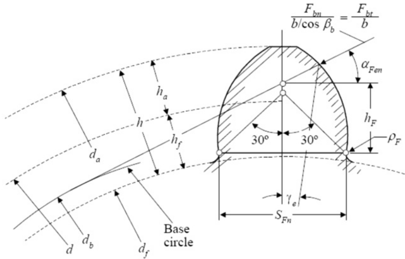
Figure 7.3 Measurements on cross-section of the tooth profile of a typical external cylindrical gear
