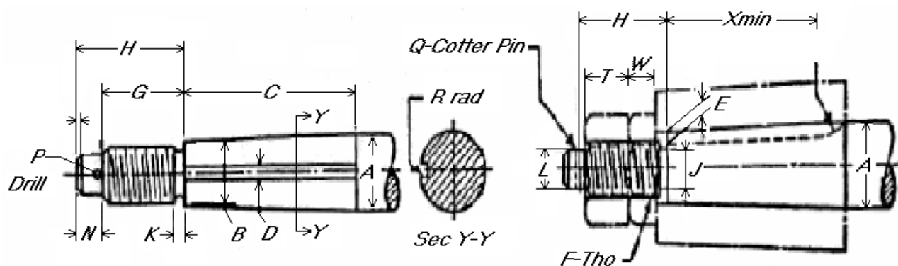
Figure 5.2 Typical details of propeller shaft ends
