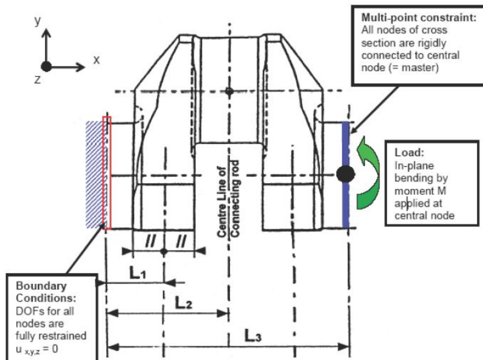
Fig. 2.9 Boundary and load conditions for the pure bending load case
