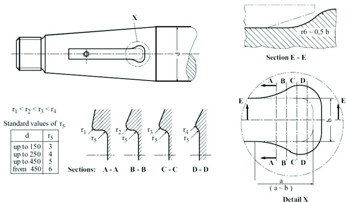
Figure 5.1 Design of keyway in propeller shaft
