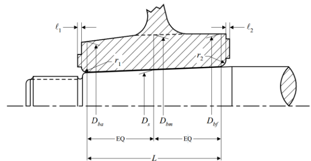
Figure 8.3 Theoretical Contact Surface Between Hub and Shaft
