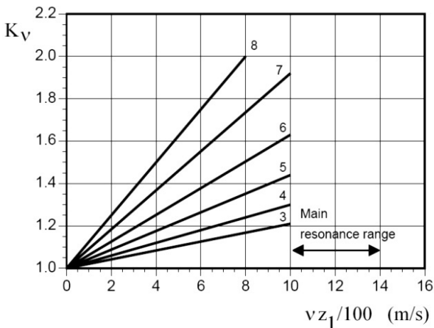
Figure 7.2 Dynamic factor for spur gears
