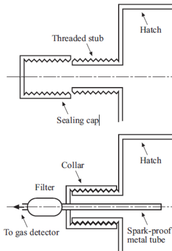
Fig. 12.2 Gas sampling points
