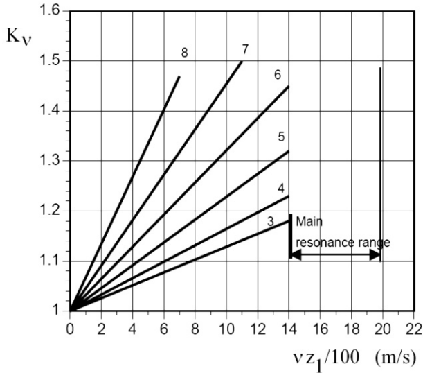
Figure 7.1 Dynamic factor for helical gears
