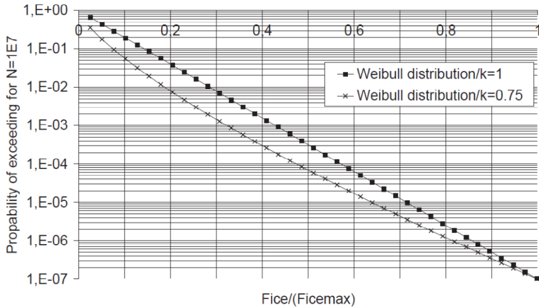
Figure 19.2 The Weibull-type distribution (probability that F_{ice} exceeds a portion of (F_{ice})_{max} ) that is used for fatigue design.
