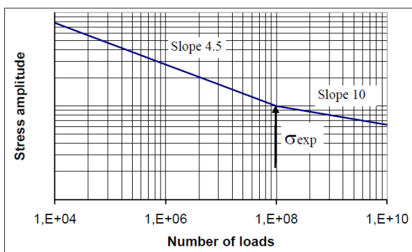
Figure 19.4 Two-slope S-N curve
