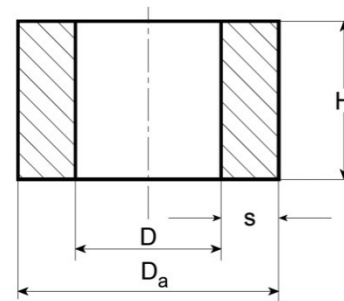
Figure 9.1 Hub dimensions
