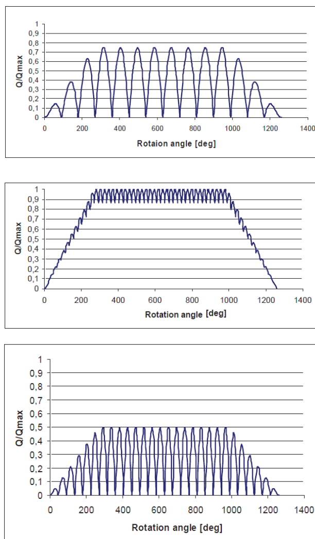
Figure 19.3. The shape of the propeller ice torque excitation for 90, and 135 degree single-blade impact sequences and 45 degree double blade impact sequence. (Figures apply for propellers with 4 blades.)
