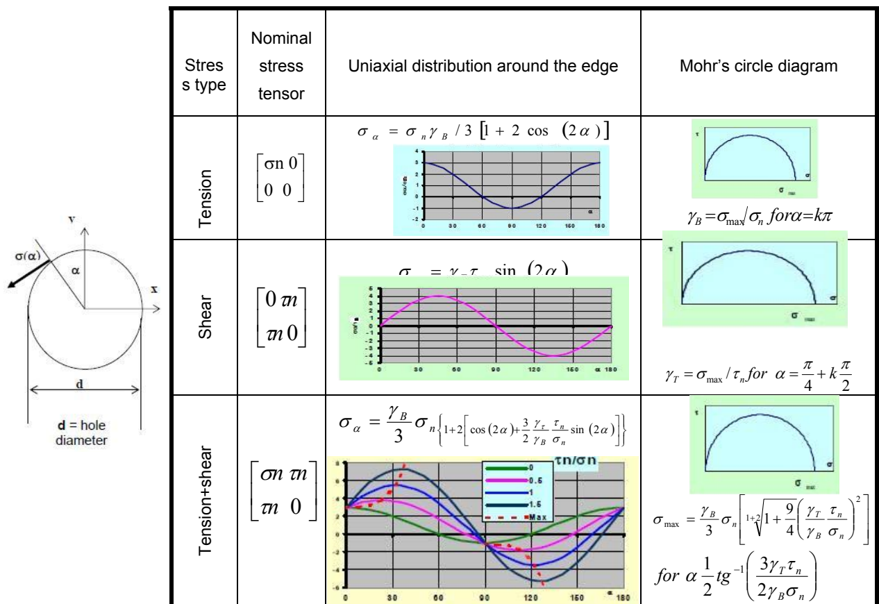
Fig. 2.14 Stress concentration factors and stress distribution at the edge of oil drillings
