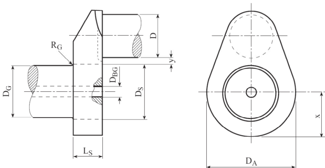
Fig. 2.12 Crank throw of semi-built crankshaft
