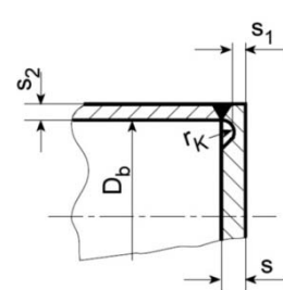
Figure 12.17 Welded-neck endplates with relieving groove
