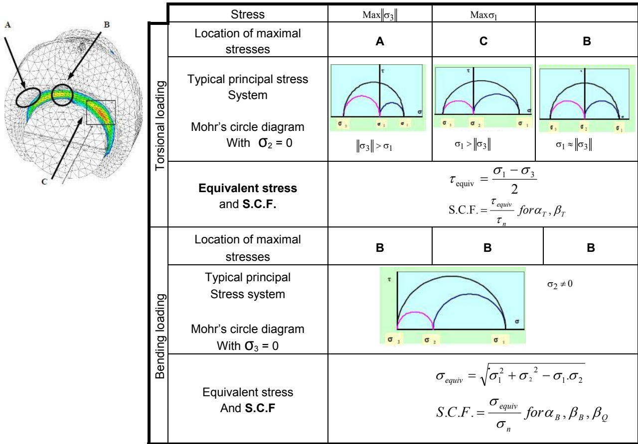
Fig. 2.13 Definition of stress concentration factors in crankshafts fillets
