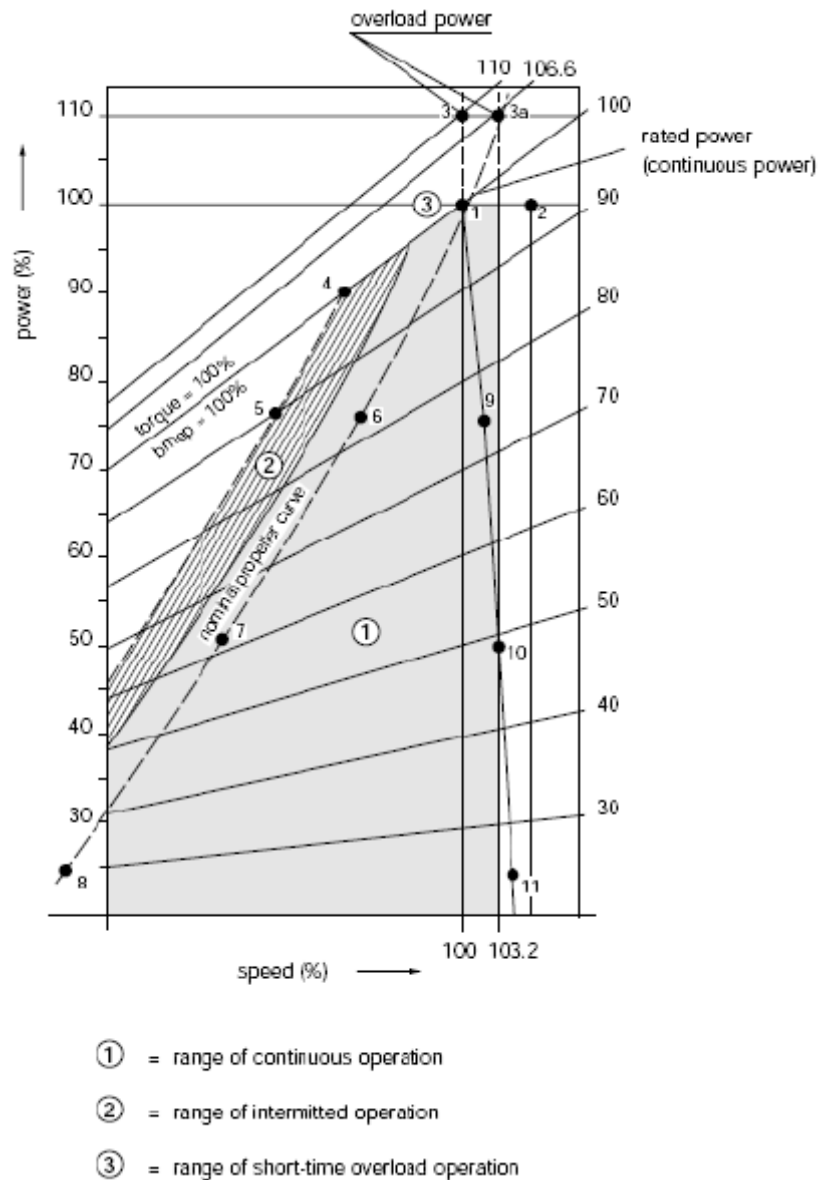
Fig. 2.15 – Load points
