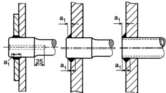
Figure 12.22 Figure 12.23 Figure 12.24 Parameters for welding of stays, stay tubes and stay bolts
