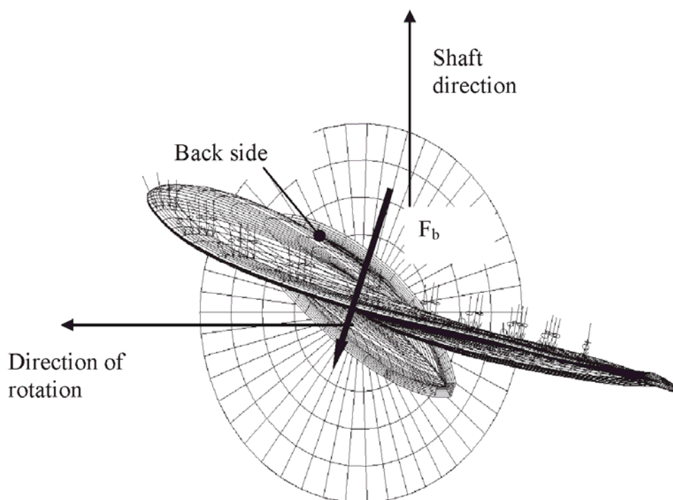
Figure 19.1 Direction of the backward blade force resultant taken perpendicular to chord line at radius 0.7R. Ice contact pressure at leading edge is shown with small arrows.
