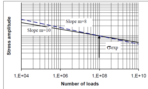
Figure 19.5 Constant-slope S-N curve
