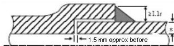
Figure 16.2 Typical Socket Weld Joint
