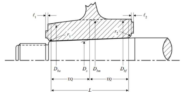
Figure 8.3 Theoretical Contact Surface Between Hub and Shaft
