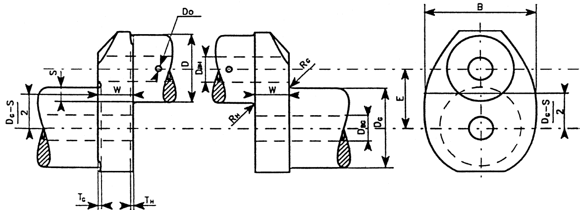
Fig. 7 – Crank dimensions
