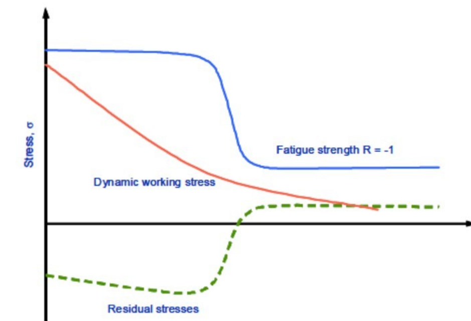
Figure 3.1. Stresses as functions of depth, general principles
