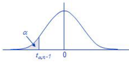
Figure 2.1. Student's t -distribution
