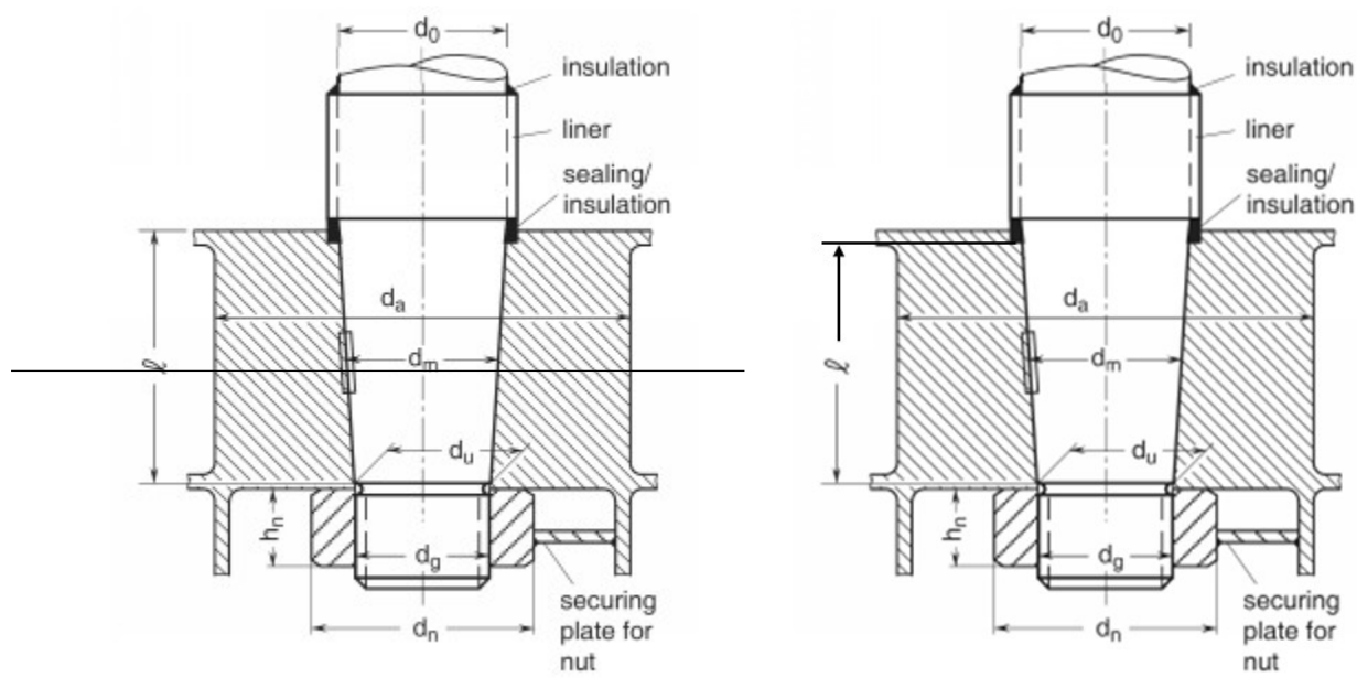
Figure 5 Cone coupling with key
