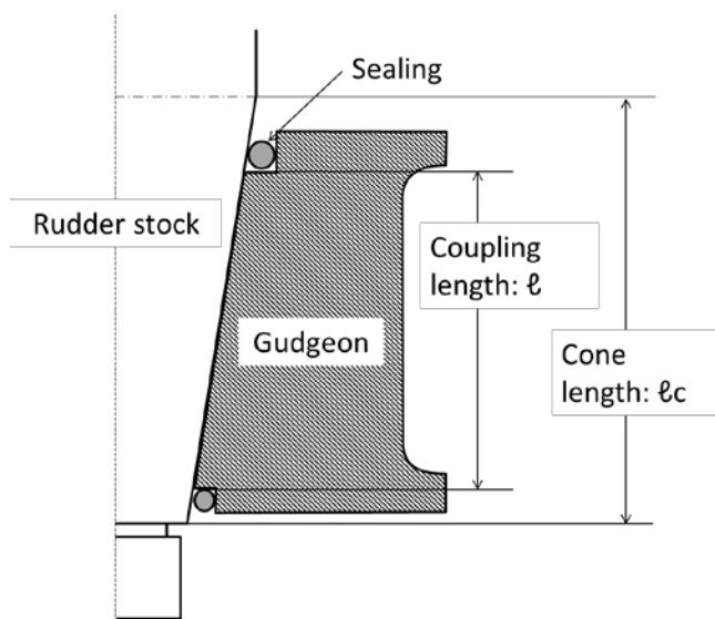
Figure 5b Cone length and coupling length
