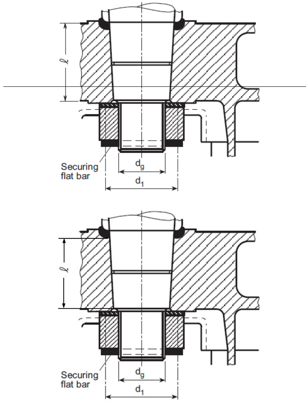
Figure 6 Cone coupling without key
