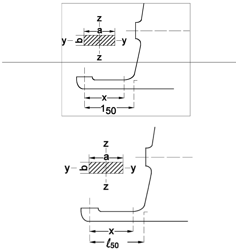
Figure 7 Sole piece
