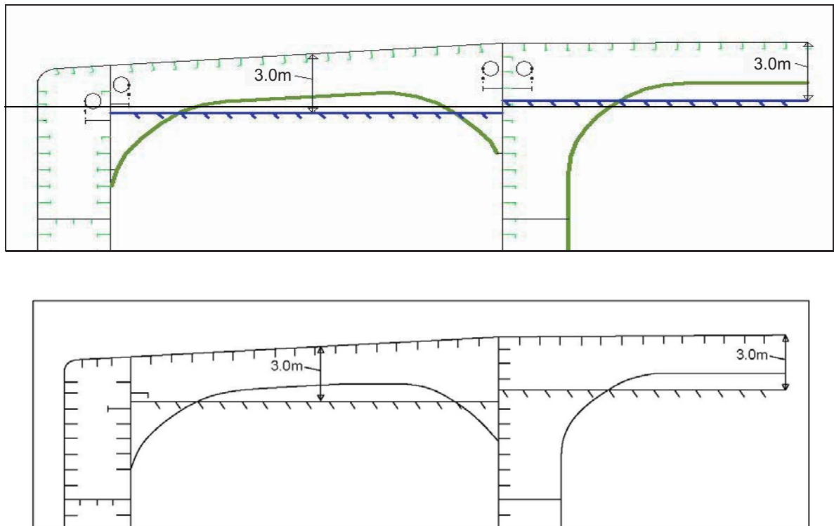
Figure 4 Maximum water level in a tank
