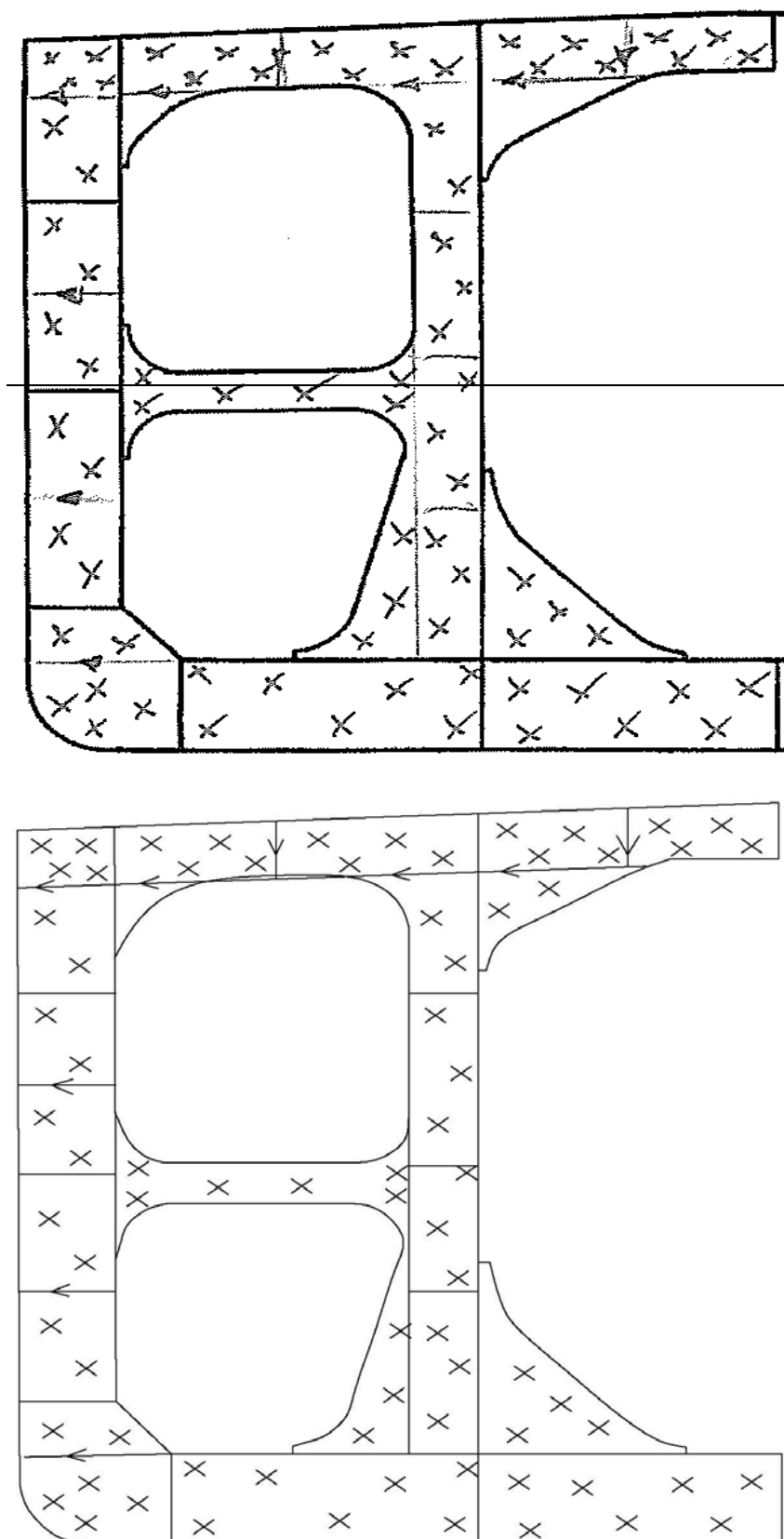
Figure 6 - Transverse rings in cargo and ballast tanks
