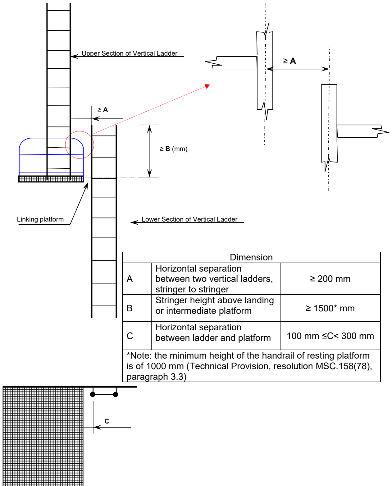
Figure “B” Vertical Ladder – Side mount
