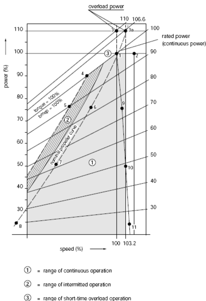
Figure 1 Load points
